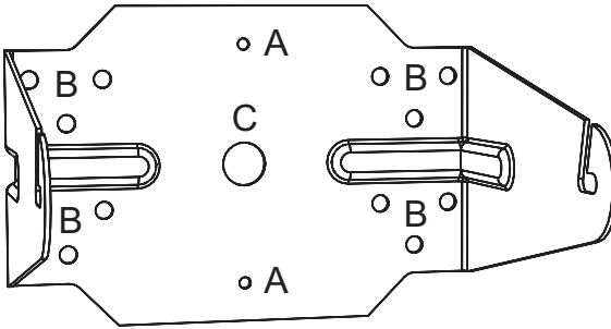
Horizontal mounting
