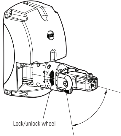
Vertical adjustment
