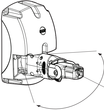
Horizontal adjustment
