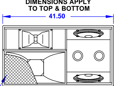
FRONT GRILLE PARTIALLY SHOWN
