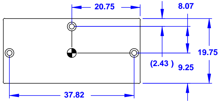
TOP DIMENSIONS APPLY TO TOP & BOTTOM
