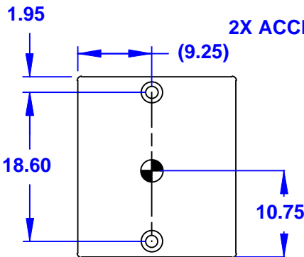
SIDE DIMENSIONS APPLY TO BOTH SIDES
