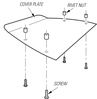
1. ASSEMBLING END COVER
