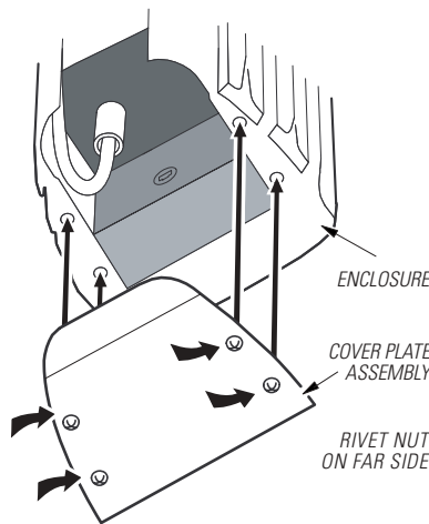
2. END PLATE INSTALLATION
