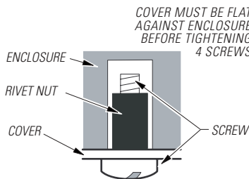
3. BEFORE TIGHTENING
