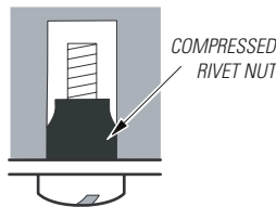
4. AFTER TIGHTENING
