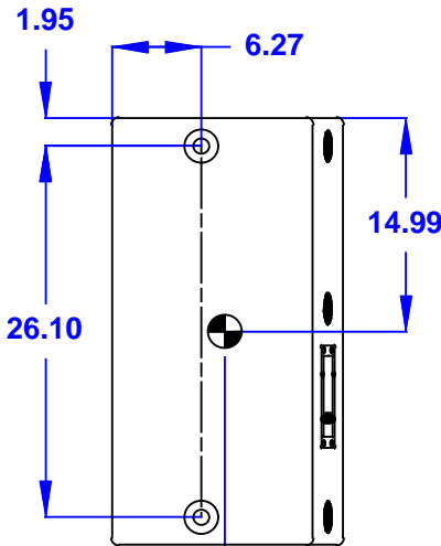
VIEW A-A DIMENSIONS APPLY TO BOTH SIDES
