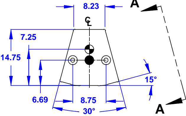
TOP DIMENSIONS APPLY TO TOP & BOTTOM
