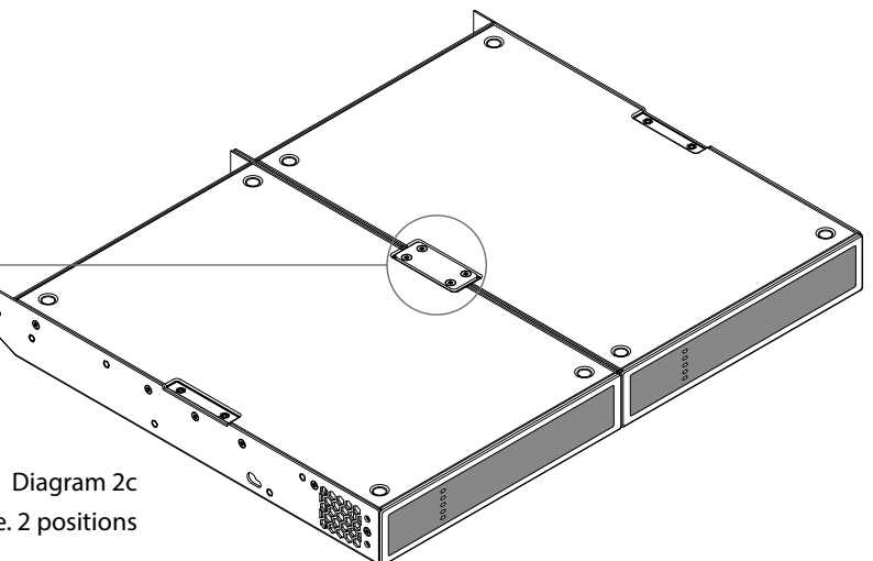
Connection Plate + 4 x M3 x 6 countersunk
