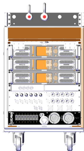
UXR FRONT PANEL VIEW
